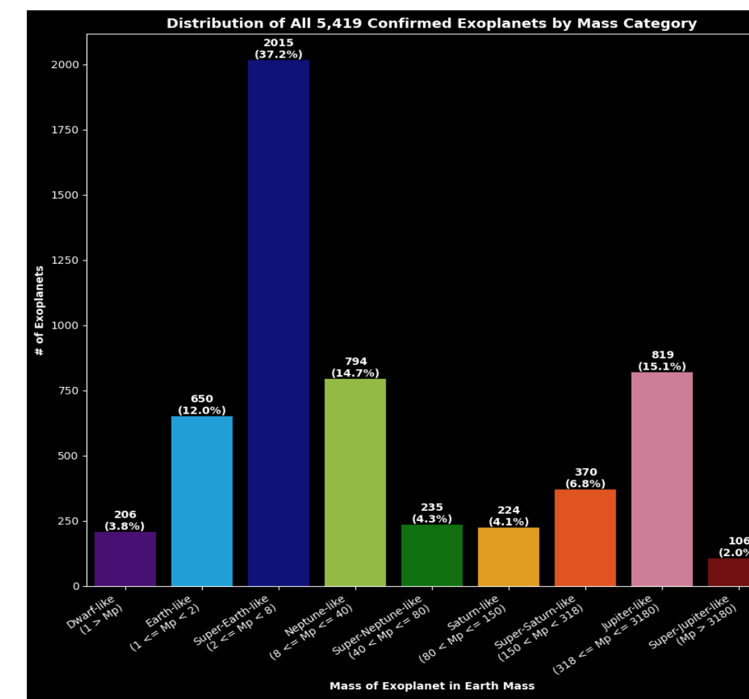
Figure 19: Bar Chart of Mass Characterization for all 5,419 Exoplanets which orbits a Main Sequence (V), Sub Giant (IV), Red Giant (III) Host Star.
